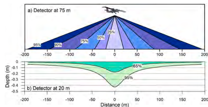
Fig. 2. Field of view (FOV) of an airborne measurement. Not true scale. (a) Detector at 75 m (aircraft), percentage radial contributions to the measurement. (b) Detector at 20 m (drone), after van der Veeke et al. (2021), subsurface contributions (65% and 95%) to the measurement.
