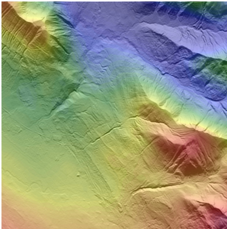
Scanning LiDAR digital terrain with magnetic data superimposed
